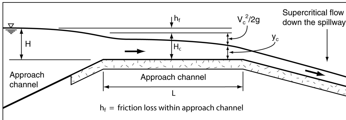
Figure A14 – Hydraulic profile for a spillway where friction loss within the approach channel is significant
