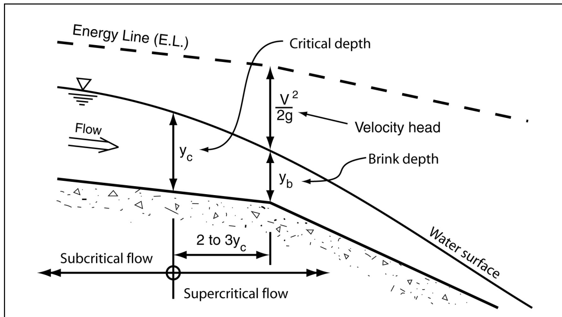
Figure A10 – Water passing through critical velocity as it enters a steep Chute
