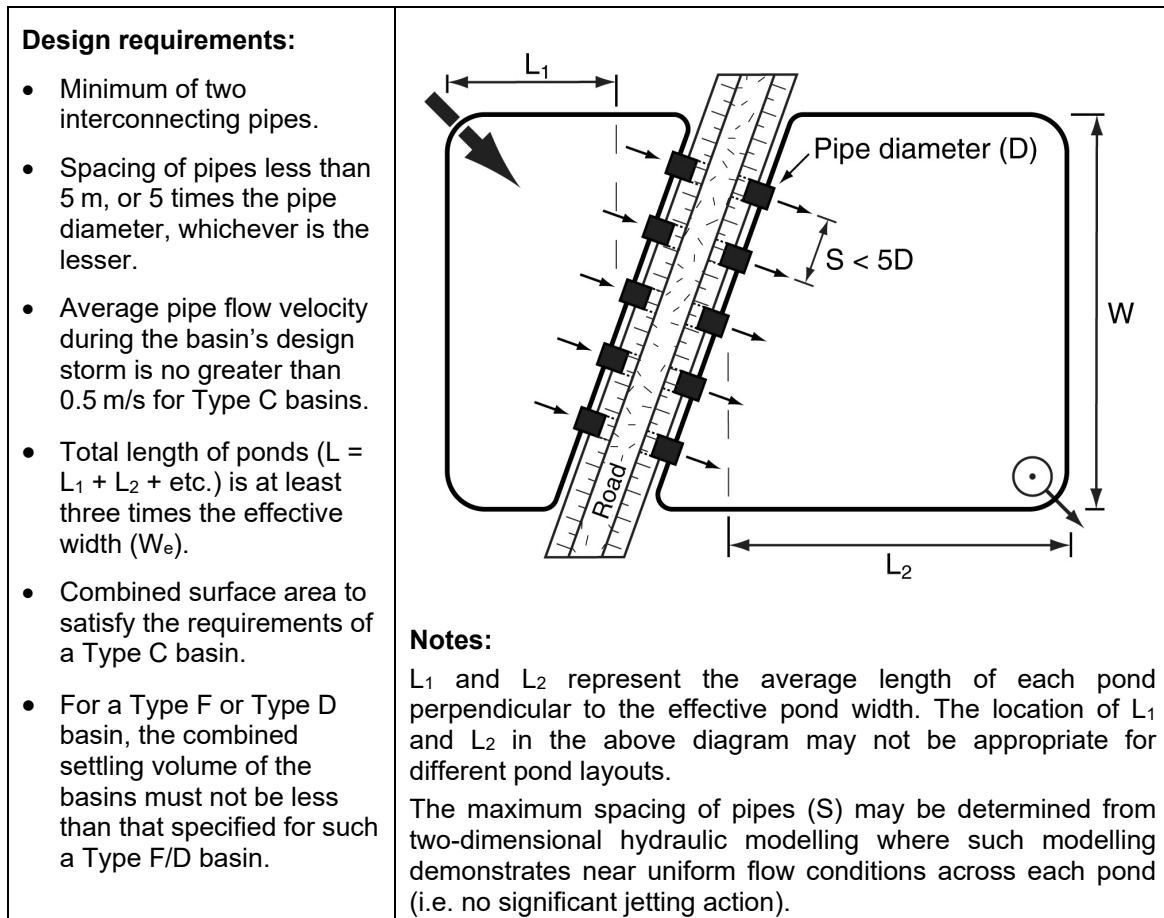
Figure B3 – Multiple Sediment Basins with multiple connecting pipes
