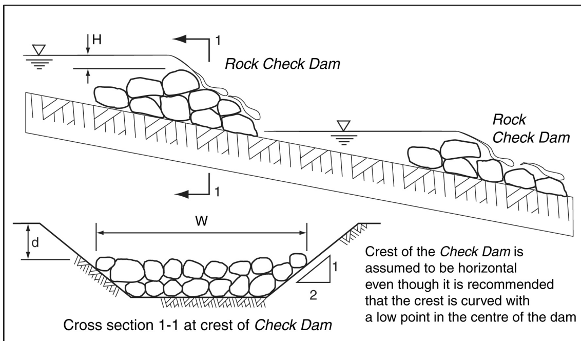
Figure A15 – Assumed hydraulics of a Check Dam
