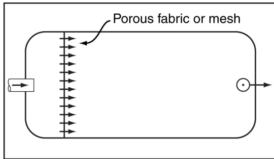
Figure B9(a) – Porous barrier inlet chamber
