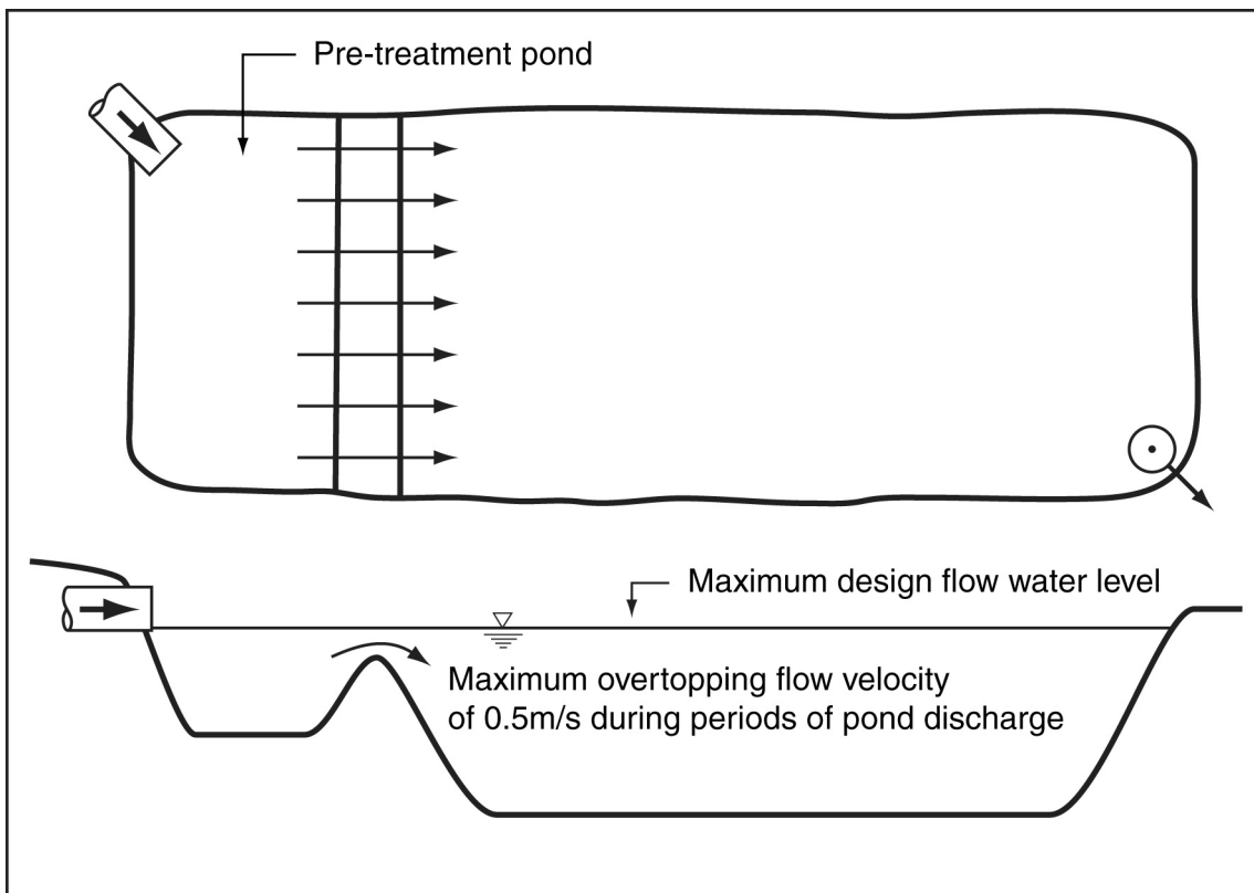
Figure B19 – Pre-treatment inlet pond
