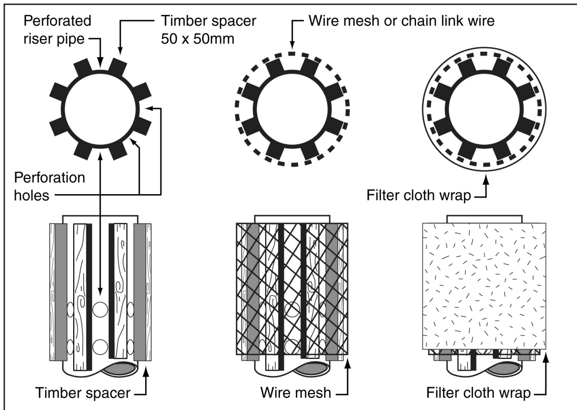
Figure B23 – Typical assembly of riser pipe with filter fabric
