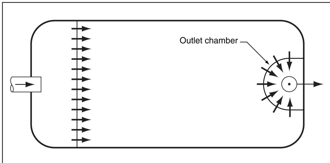
Figure B15 – Typical arrangement of outlet chamber (plan view)
