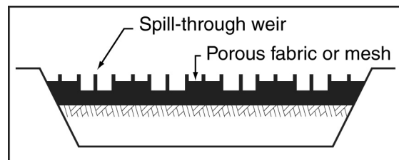
Figure B12(b) – Barrier with multiple spill-through weirs
