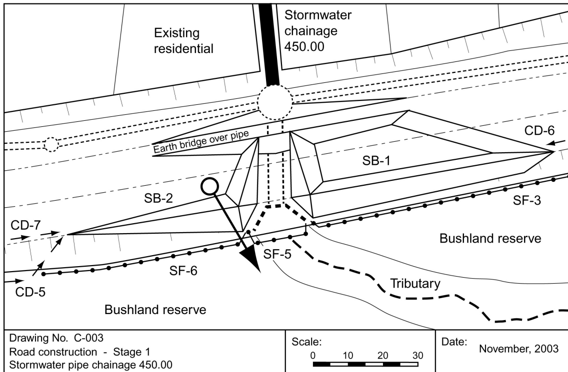
Figure D12 – Details of sediment basins (Dwg C-003)
