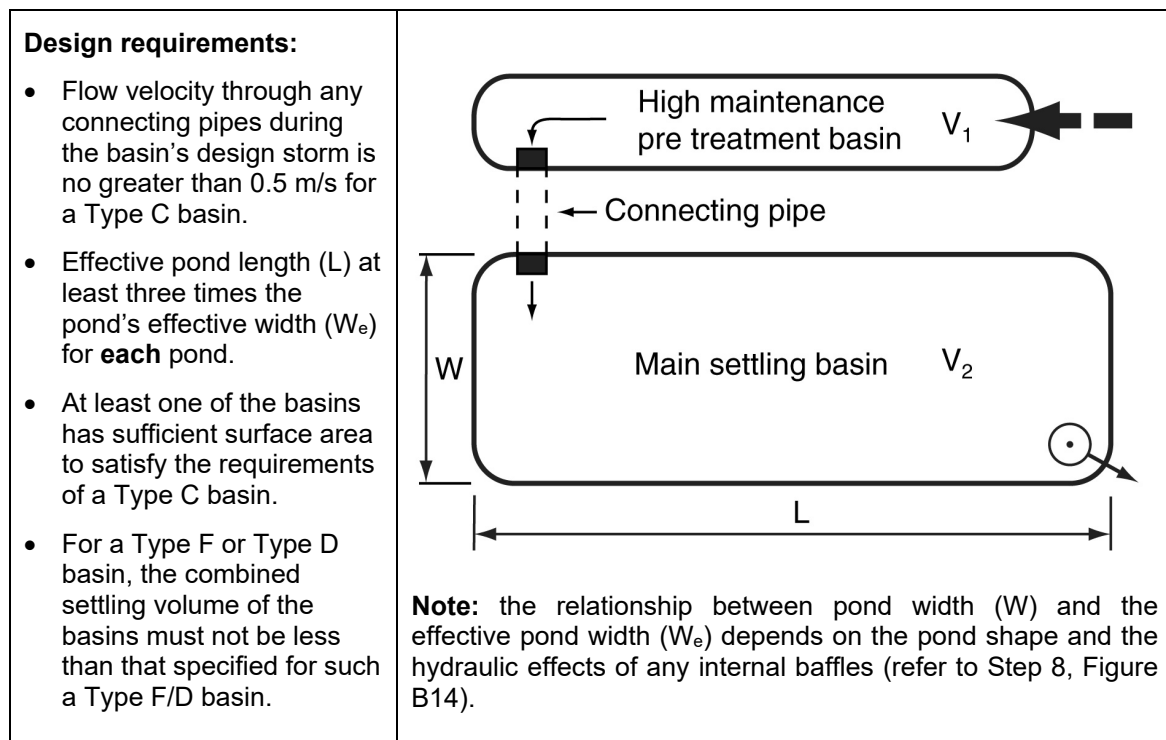
Figure B2 – Multiple Sediment Basins with single connecting pipe/culvert
