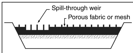
Figure B11(b) – Barrier with single spill-through weir per barrier
