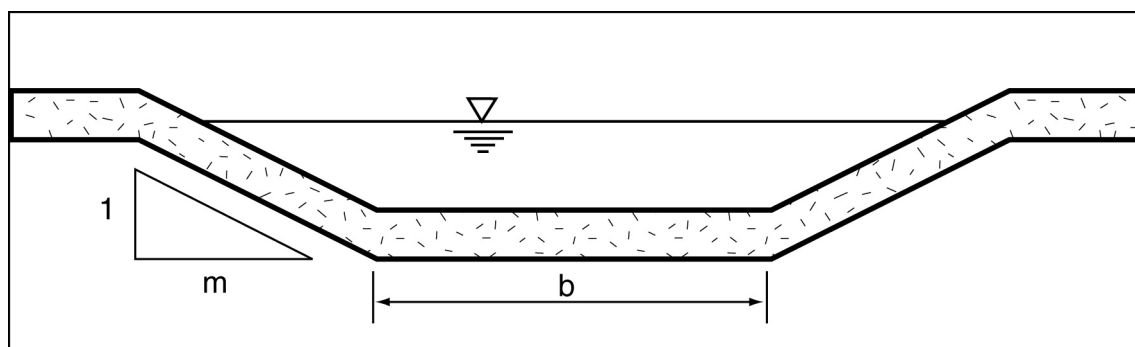
Figure A13 – Trapezoidal spillway (weir) crest
