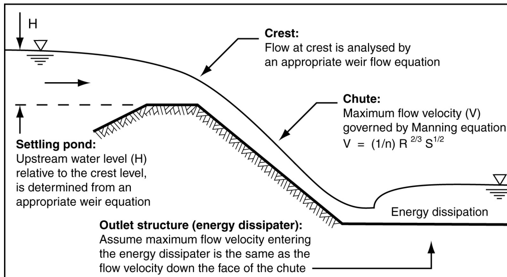
Figure A17 – Key design parameters for Chutes and spillways
