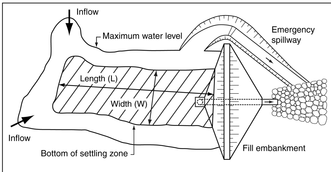
Figure B6 – Type C Sediment Basin with riser pipe outlet (plan view)
