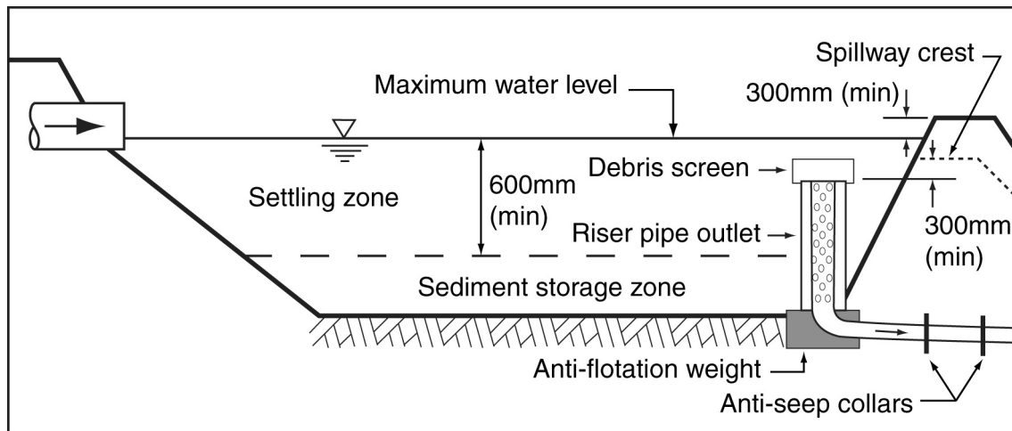
Figure B5 – Type C Sediment Basin with riser pipe outlet (long section)
