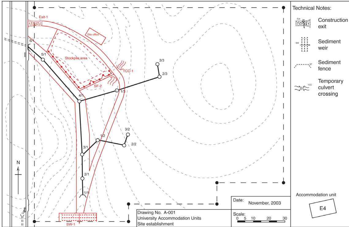
Figure D3 – Site establishment and drainage works
