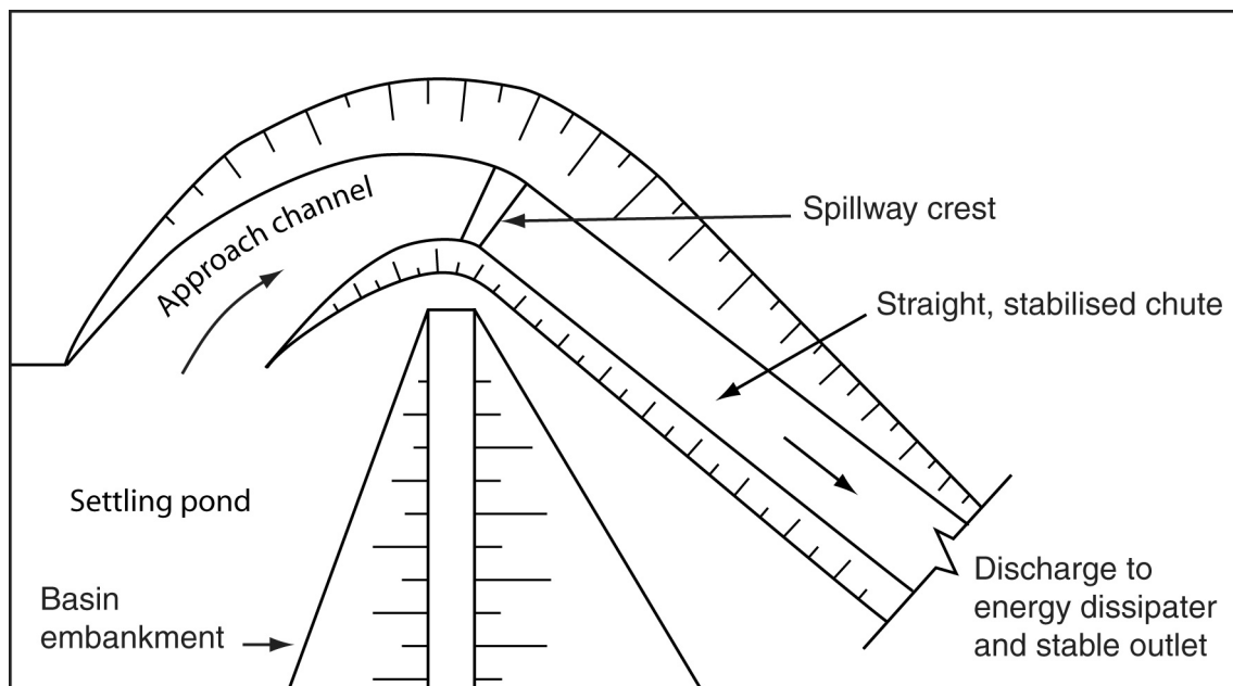
Figure A11 – Typical layout for an emergency spillway adjacent an earth fill Sediment Basin embankment
