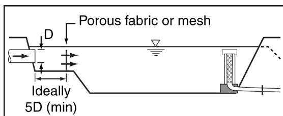
Figure B9(b) – Typical layout of inlet chamber with opposing inlet pipe (Type C basin)
