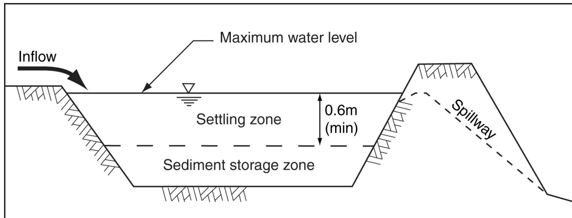
Figure B8 – Settling zone and sediment storage zone
