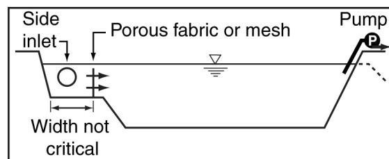
Figure B10(b) – Typical layout of inlet chamber with side inlet (Type F basin)
