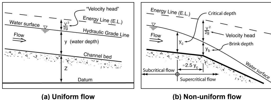
Figure A7 – Example of uniform and non-uniform open channel flow
