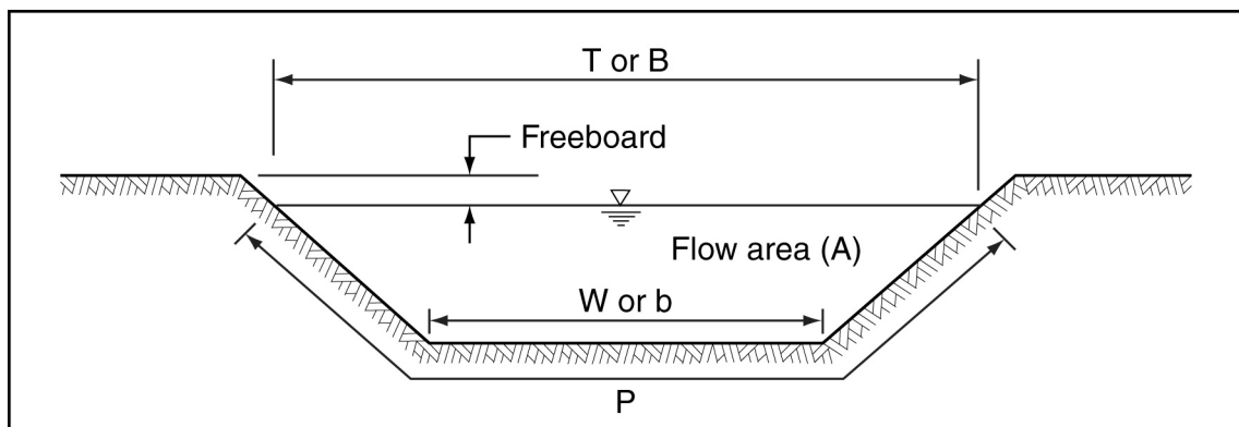
Figure A8 – Channel cross section terminology
