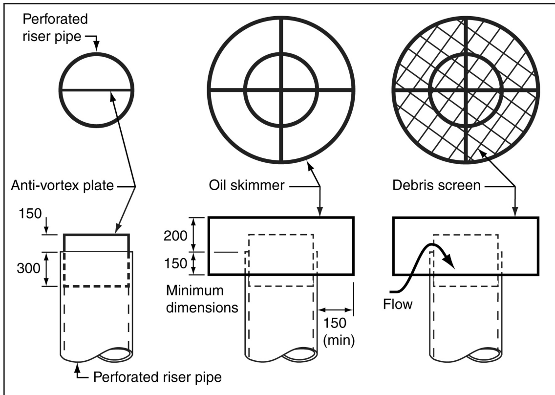
Figure B24 – Typical details of anti-vortex plate, oil skimmer and debris screen
