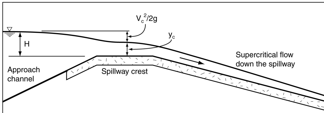
Figure A12 – Hydraulic profile for spillway crest where friction loss within the approach channel is insignificant
