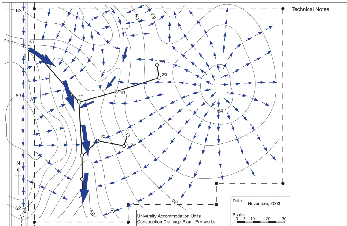
Figure D2 – Site drainage prior to development
