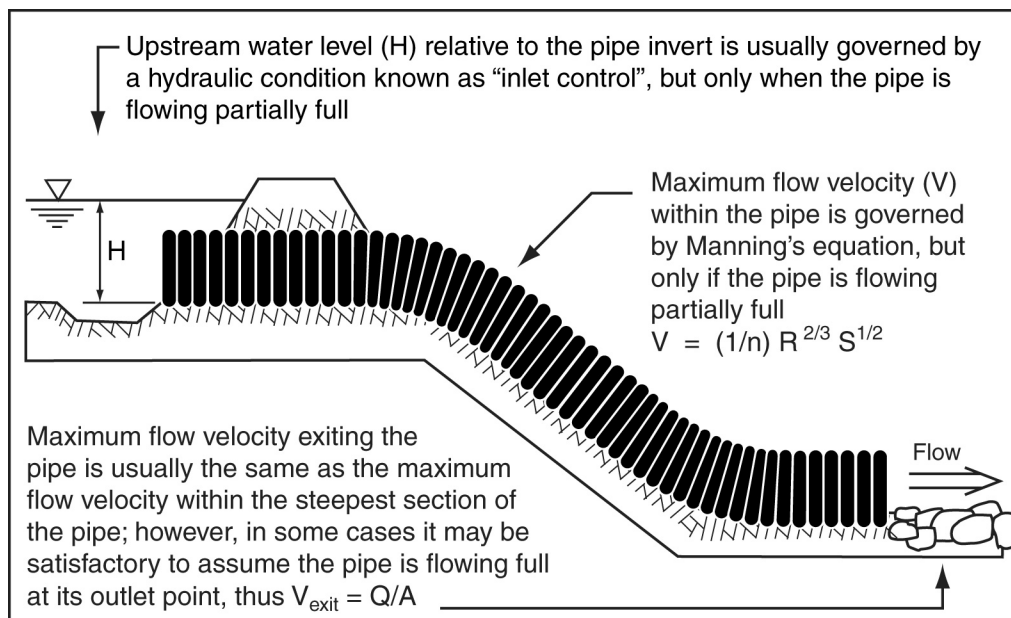
Figure A18 – Key design parameters for a Slope Drain
