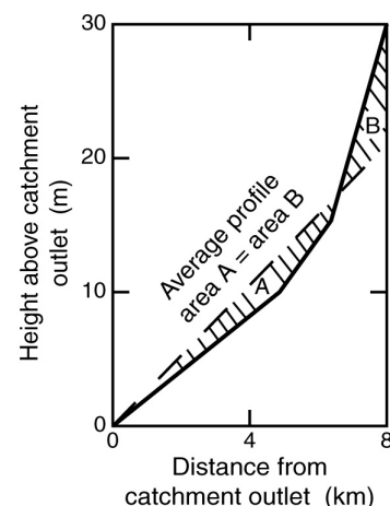
Figure A4 – Derivation of equal area slope ( S_e )
