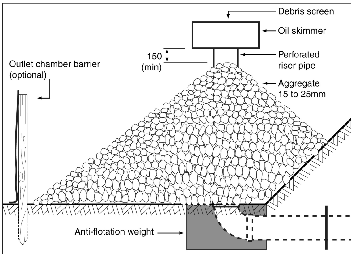
Figure B21 – Typical details of riser pipe outlet with aggregate filter
