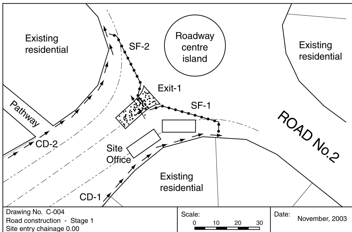
Figure D13 – Details of road intersection (Dwg C-004)
