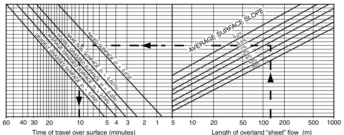
Figure A3 – Overland sheet flow times – shallow sheet flow only (sourced from ARR-1977)
