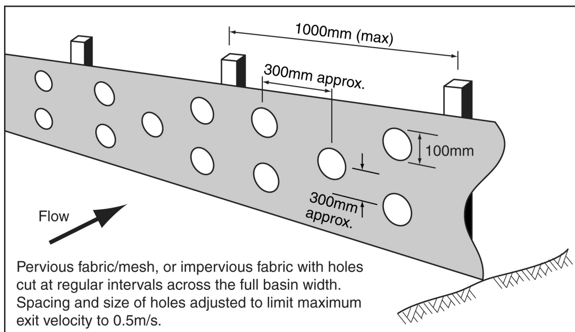
Figure B13 – Example arrangement of perforated fabric inlet baffle
