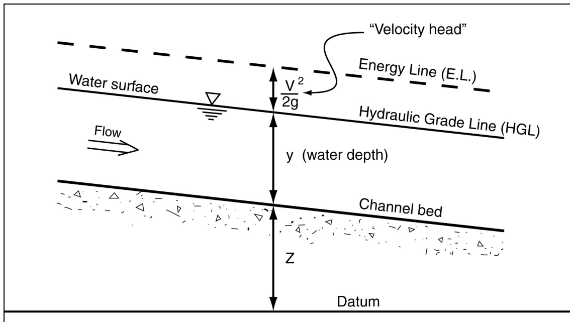
Figure A9 – Uniform flow conditions
