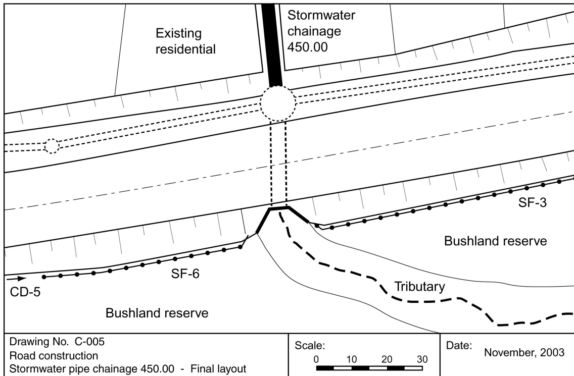
Figure D14 – Final road layout at chainage 450.00 (Dwg C-005)
