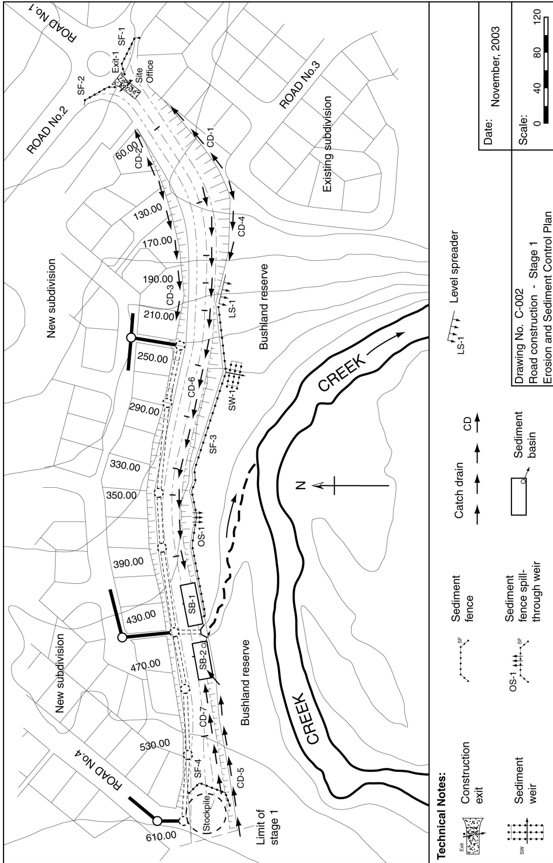
Figure D11 – Erosion and Sediment Control Plan (Dwg C-002)
