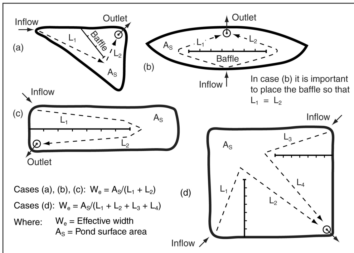
Figure B14 – Typical arrangement of internal flow control baffles (after USDA, 1975)
