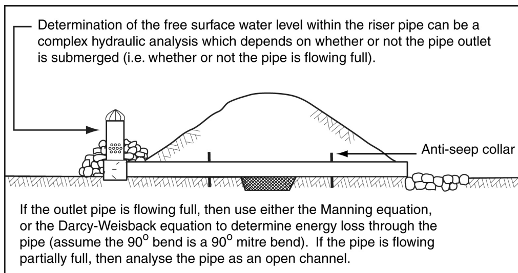
Figure A19 – Key design parameters for a Sediment Basin riser pipe outlet
