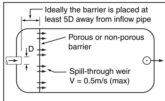
Figure B12(a) – Alternative inlet chamber design
