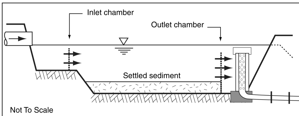
Figure B16 – Typical arrangement of outlet chamber (long section)
