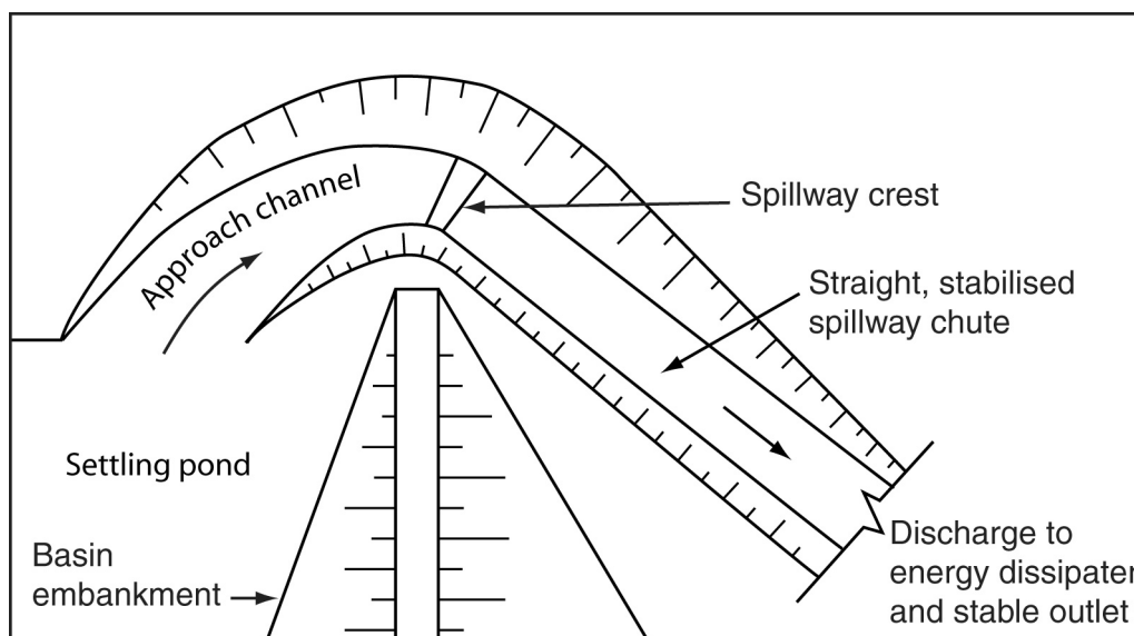
Figure B25 – Emergency spillway
