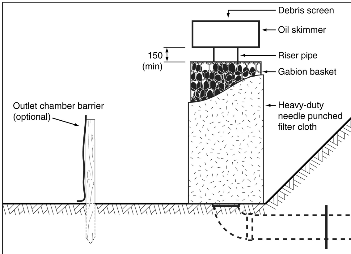
Figure B22 – Typical details of riser pipe outlet with rock-filled gabion baskets
