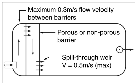
Figure B11(a) – Alternative inlet chamber design
