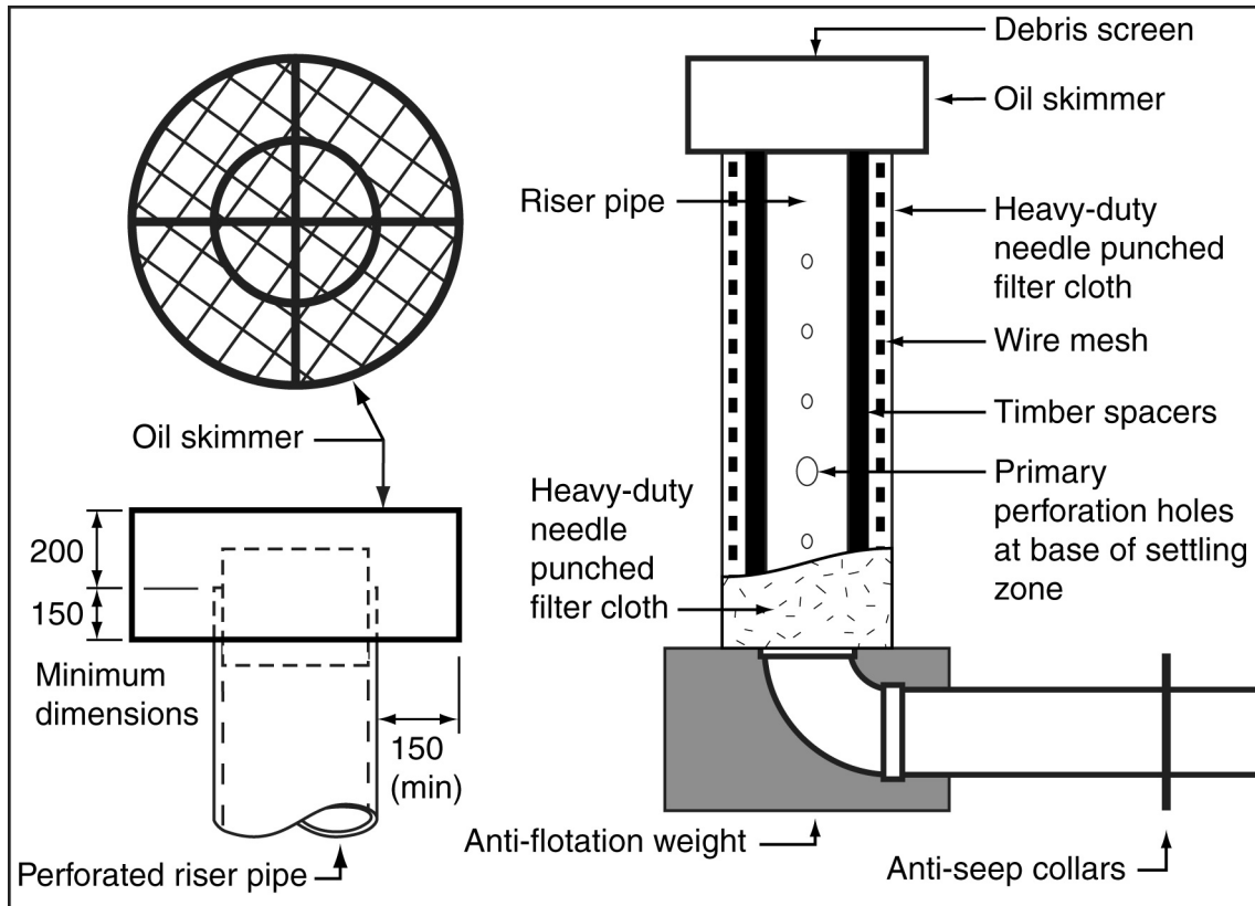
Figure B20 – Typical details of riser pipe outlet with fabric filter
