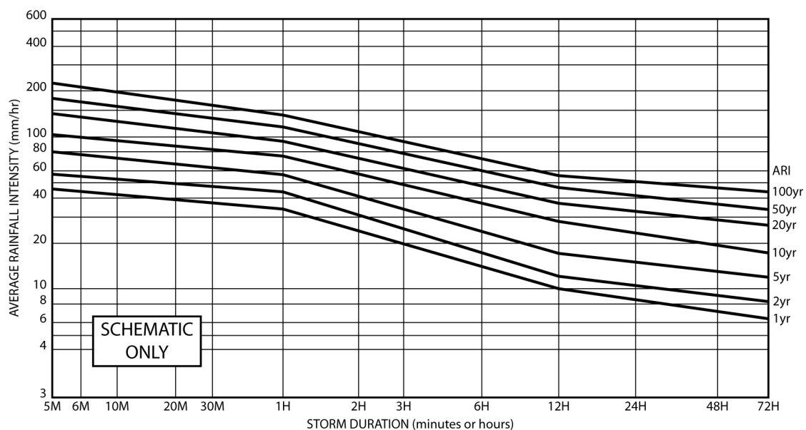
Figure A2 – Typical rainfall intensity-frequency-duration (IFD) chart
