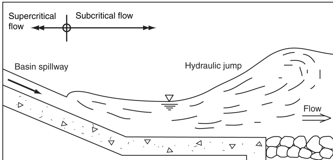
Figure A16 – Hydraulic jump at base of Sediment Basin spillway
