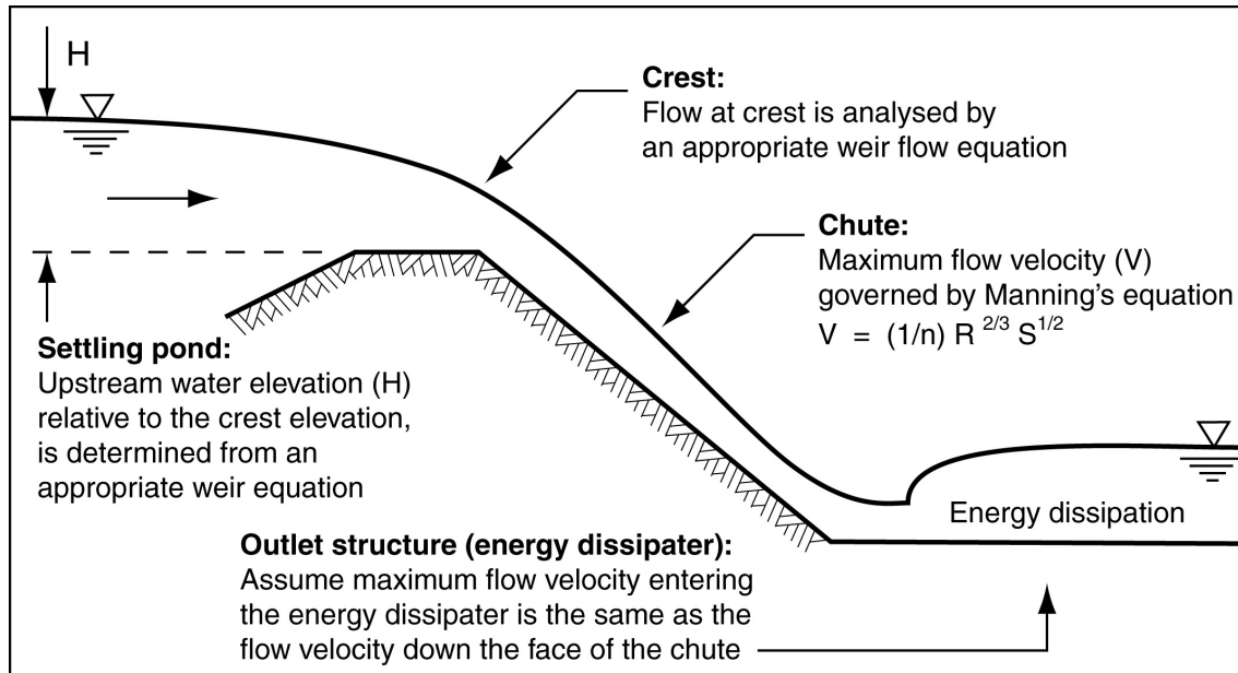
Figure B26 – Hydraulics of Sediment Basin spillways
