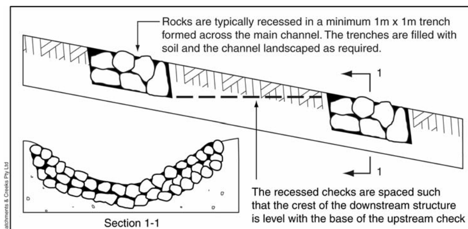
Figure 4 – Fully recessed rock check dams
