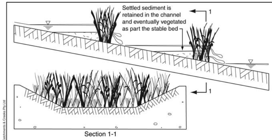
Figure 3 – Stiff grass barriers
