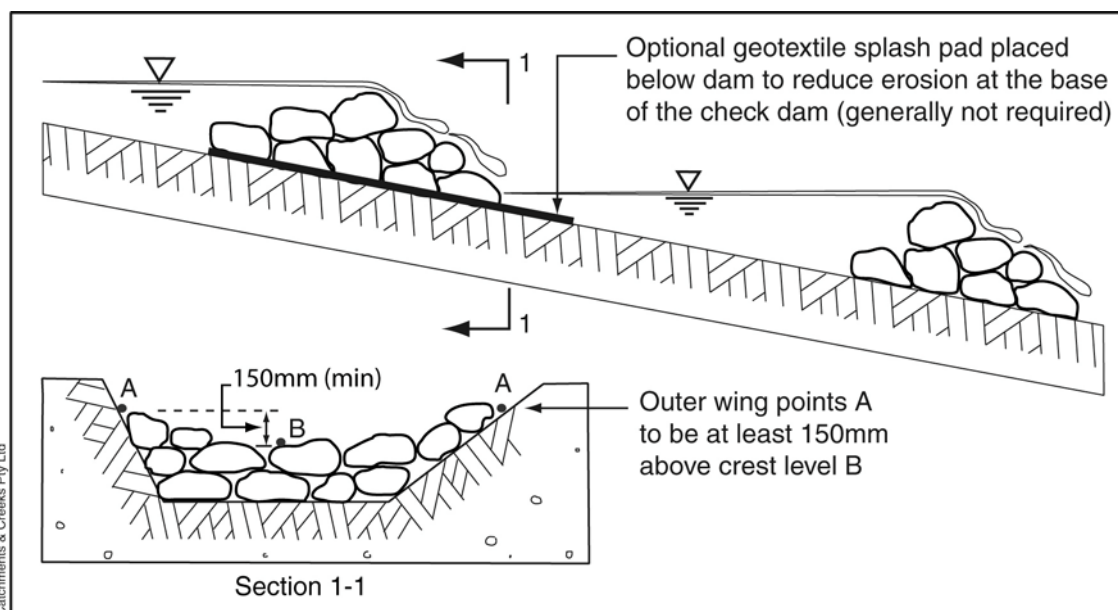
Figure 1 – Profile of temporary check dams
