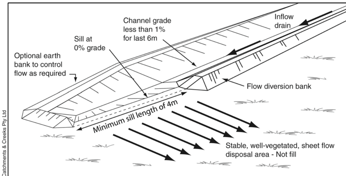
Figure 3 – Alternative level spreader layout
