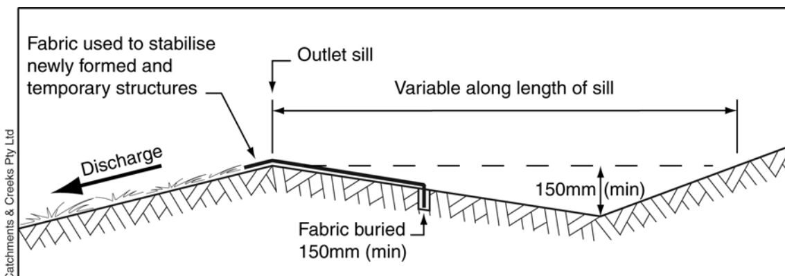
Figure 4 – Cross-sectional profile of end sill
