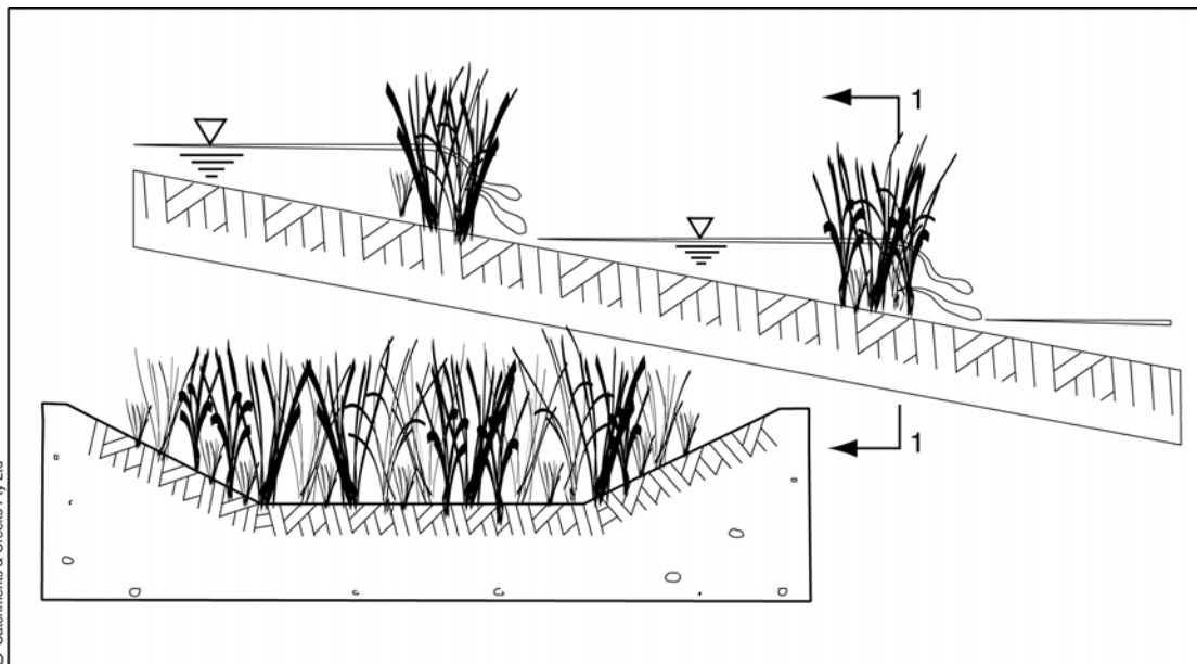
Figure 1 – Typical placement of stiff grass barriers within a drainage channel
