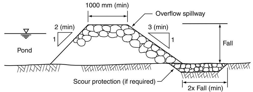
(b) Typical cross-section of rock-lined overflow spillway
