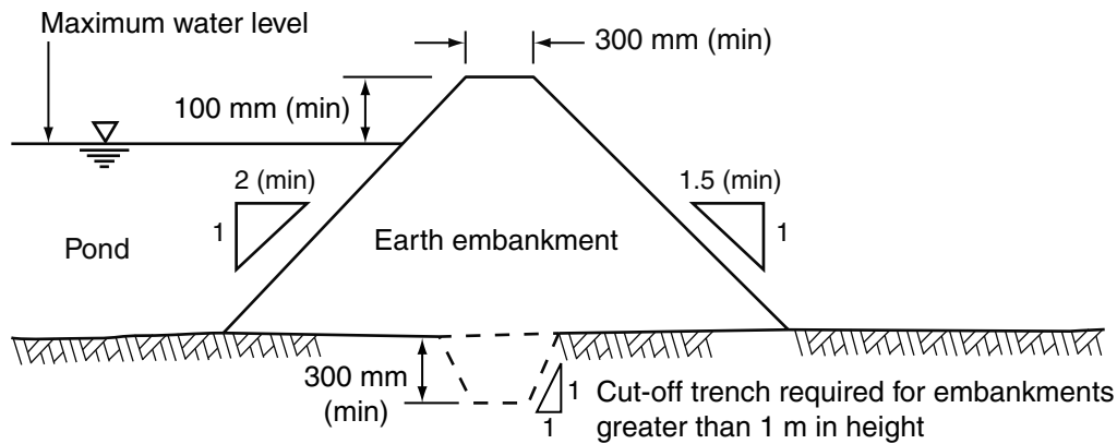
(c) Typical cross-section of earth embankment
