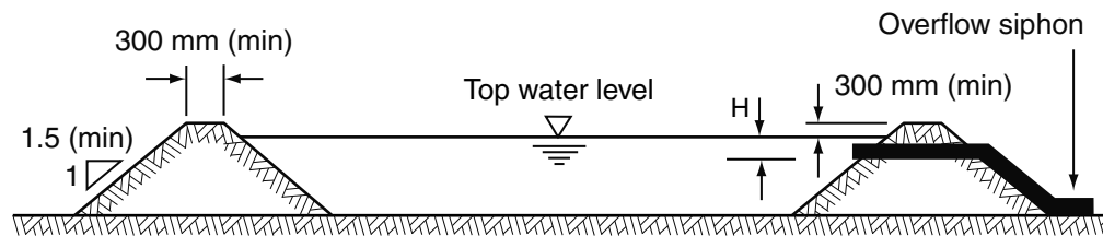
(e) Siphon overflow system
