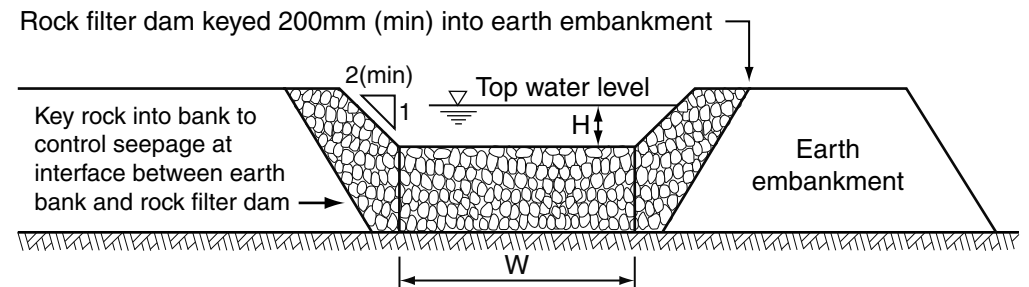
(d) Typical profile of rock-lined overflow spillway
